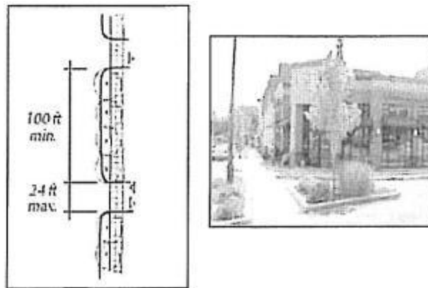
Pedestrian-friendly driveway
