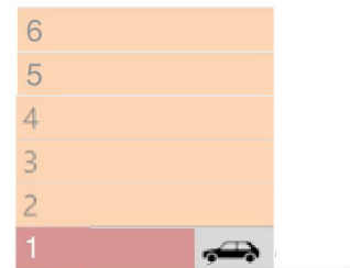
tuck-under & surface parking "5-over-1" Type III wood frame over Type I-A PT concrete podium
